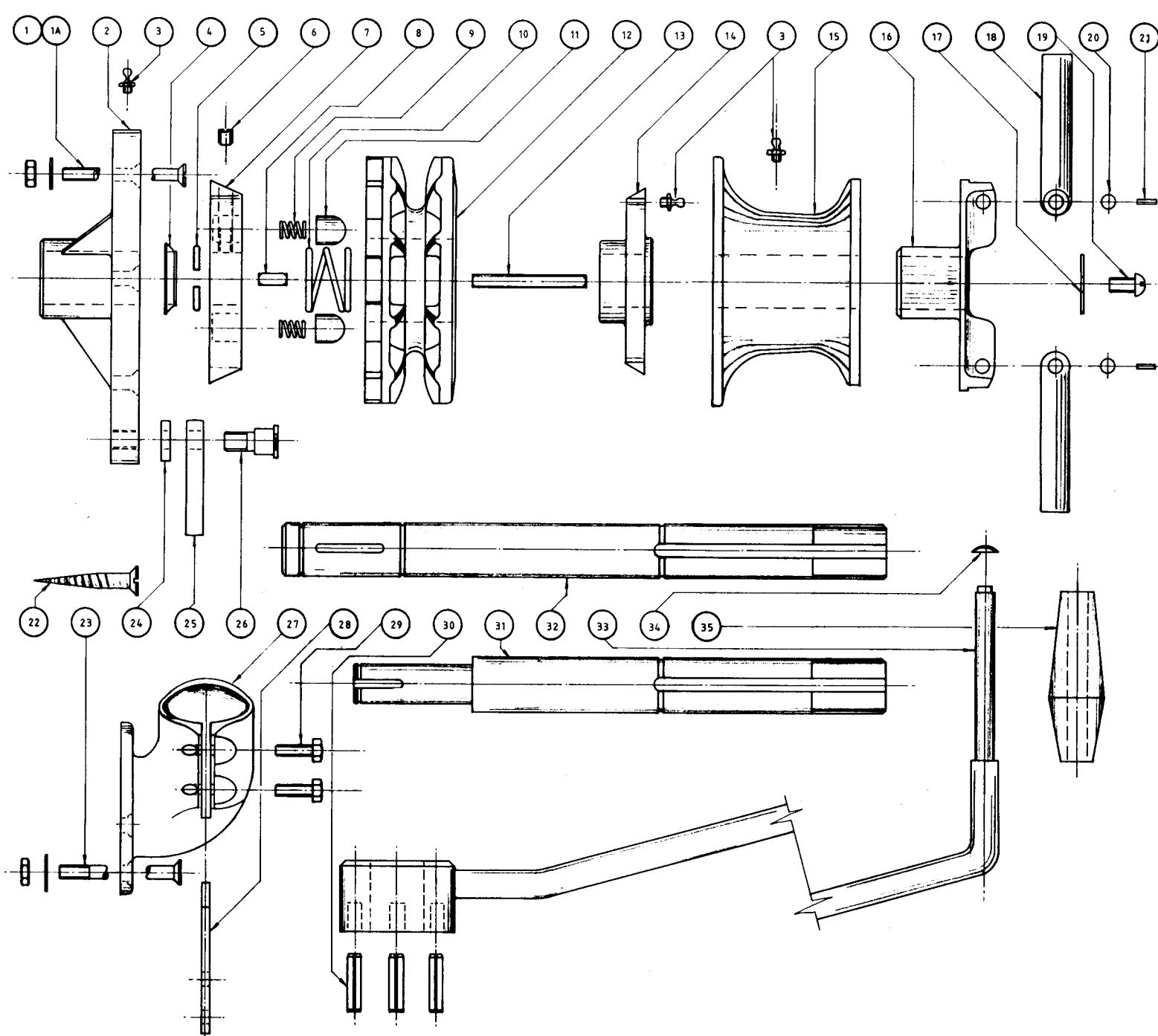
PARTS LIST FOR V 1000 & V 3000 ( ABOVE DECK COMPONENTS )
